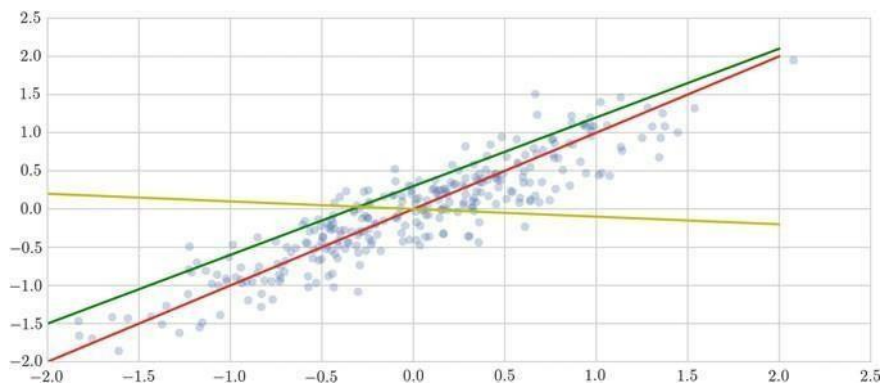
Fig. 6.1 Illustration of different simple linear regression models. Blue points correspond to a set of random points sampled from a univariate normal (Gaussian) distribution. Red, green and yellow lines are three different simple linear regression models
