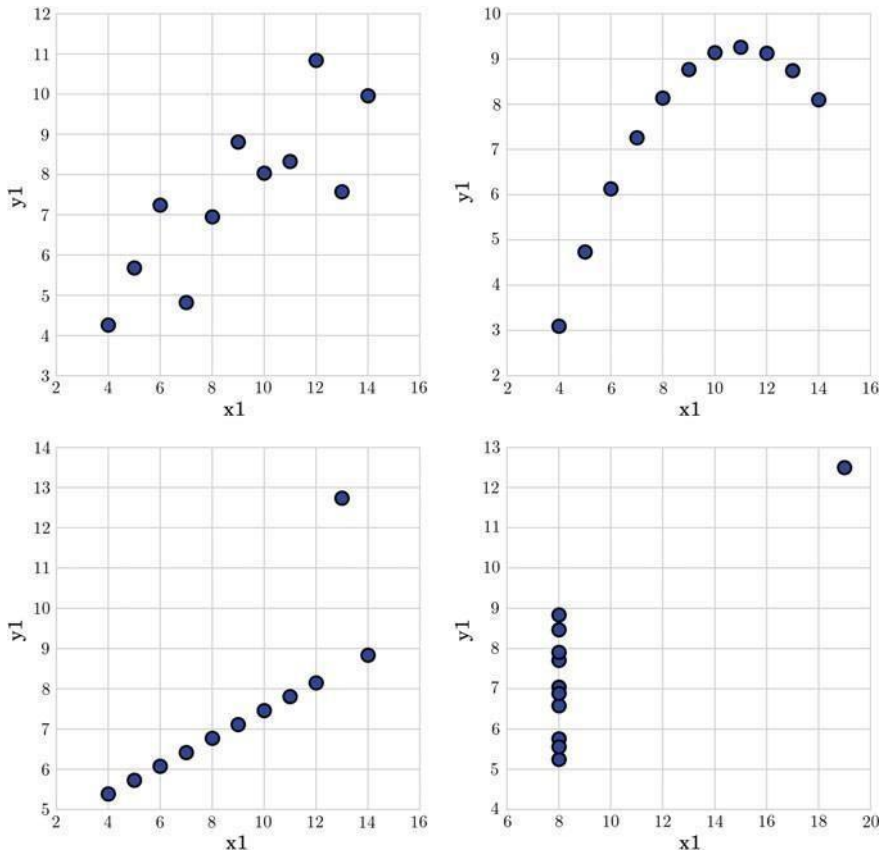
Fig. 3.10 Anscombe configurations
